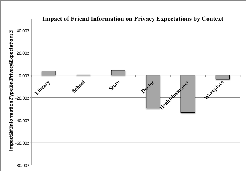
Figure 3c: Friend Information
